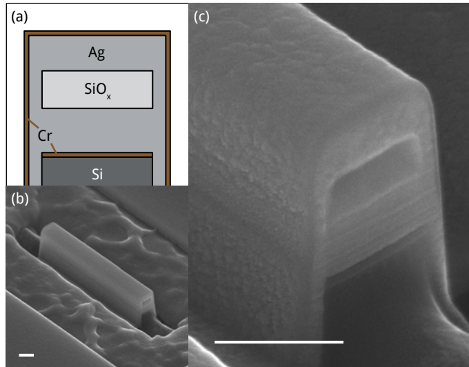
Figure 7.1: Scanning electron micrographs of a 2\text{ }\mu\text{m} long, focused-ion-beam fabricated MIM waveguide. (a) Schematic of the end facet, showing the Si/Cr/Ag/ \text{SiO}_x /Ag/Cr layer structure. (b) Finalized waveguide (c) Detail of end facet. Scale bars: 200 nm
