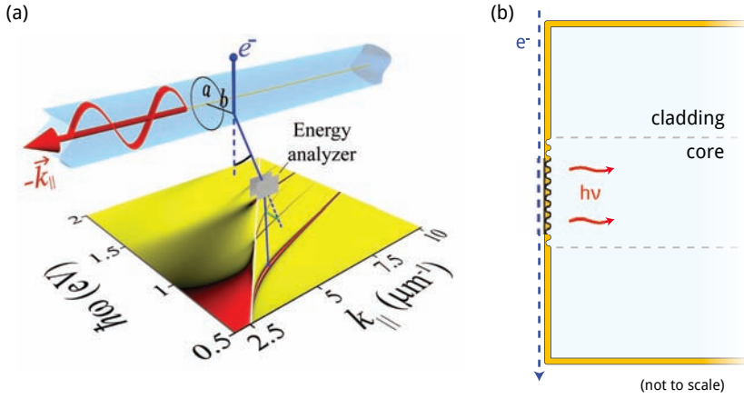
Figure 8.6: Schematic for excitation of a single photon in an optical fiber by an incoming electron. (a) (from Ref. [207]) Geometry for electrons that pass the fiber perpendicularly. As a result of coupling to a guided photon, the electron loses energy (analyzed by an electrostatic analyzer) and transfers momentum, resulting in deflection of the electron trajectory. (b) An alternative geometry consisting of an optical fiber of which the end facet is coated with a Au film. At the fiber core, a grating provides efficient coupling of the electron beam to a waveguided photon.
