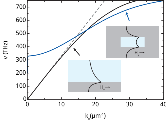
Figure 1.1: Dispersion relation of SPPs for frequencies below the surface plasmon resonance. Dashed line: light line in glass. Black curve: SPP on a Ag-glass interface. Blue curve: TM SPP in a Ag-glass-Ag waveguide with a 200 \times 85 nm core.
