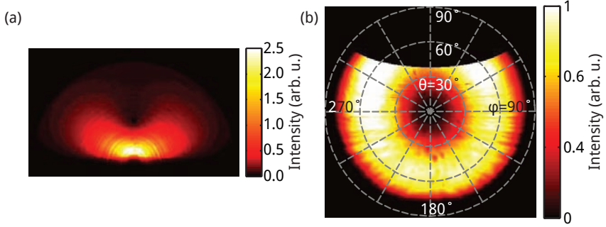
Figure 1.5: Angle-resolved CL emission recorded on a 1024 \times 1024 pixel CCD array detector. (a) Image showing the light emerging from the parabolic mirror. The emission originates from a 30 keV electron beam incident on an unstructured Au surface, giving rise to transition radiation. (b) Angular distribution of the transition radiation, obtained by transformation of the CCD image in (a). Polar ( \theta ) and azimuthal ( \varphi ) angles are indicated.
