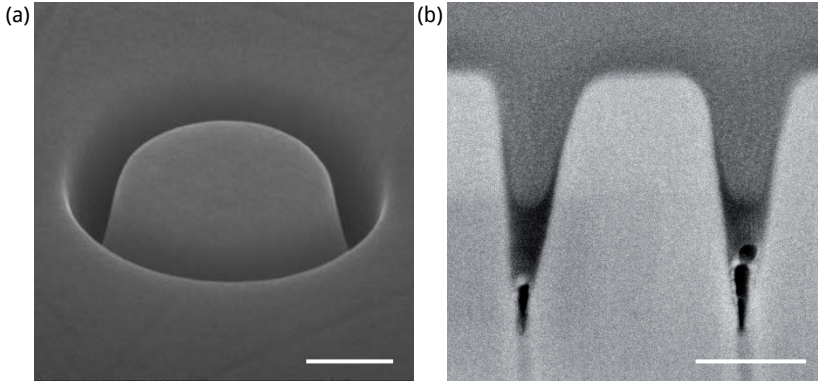
Figure 6.1: Scanning electron micrographs of plasmonic whispering gallery resonator with radius r = 300 nm and groove depth d = 500 nm. (b) FIB-milled cross-section through resonator infilled with a PVB polymer layer spin coated onto the sample surface from solution. It forms a thin ( < 50 nm) layer onto the surface and fills the bottom part of the V-groove (dark contrast). Air inclusions are formed at the bottom of the groove. Scale bars: 200 nm
